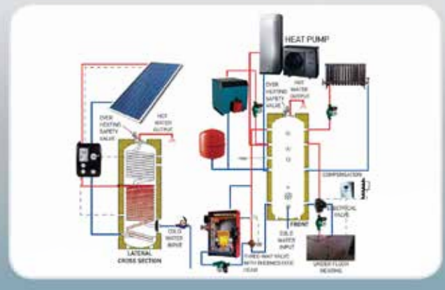
Typical Installation Buffer-1 Tank with INOX heat exchanger for Domestic Hot Water
